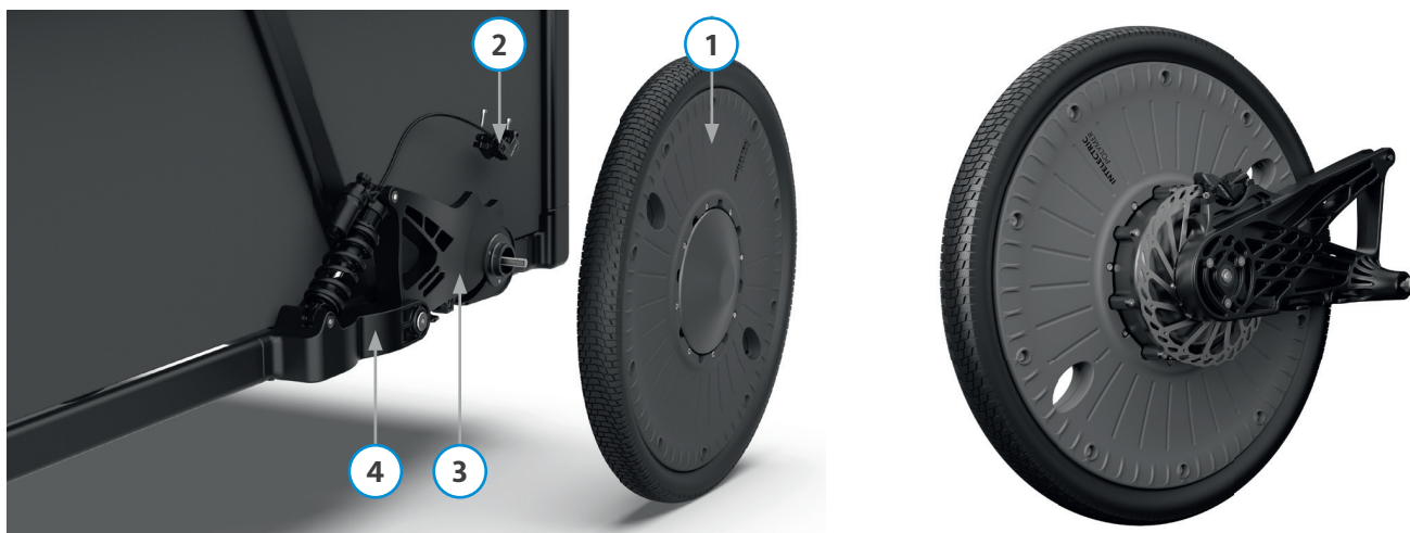
Interface to the INTELECTRA Cargobike ASM frame: ① icoMR1500.24/ ② iBRS/ ③ icoSA/ ④ ASMframe
